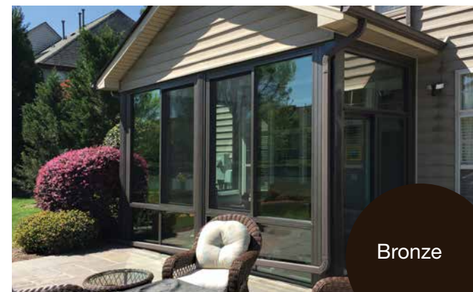
Sandstone
